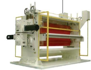
2000 Servo Drive Rotary Knife developed by Chicago Electric.
