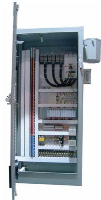
PLC & Power Section
