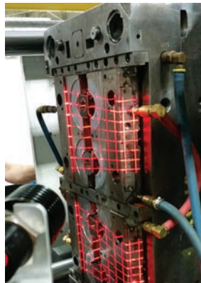
Over-mold insert inspection with LED light grid
