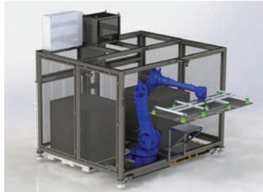
Sheet feed robot with precision vision guidance
